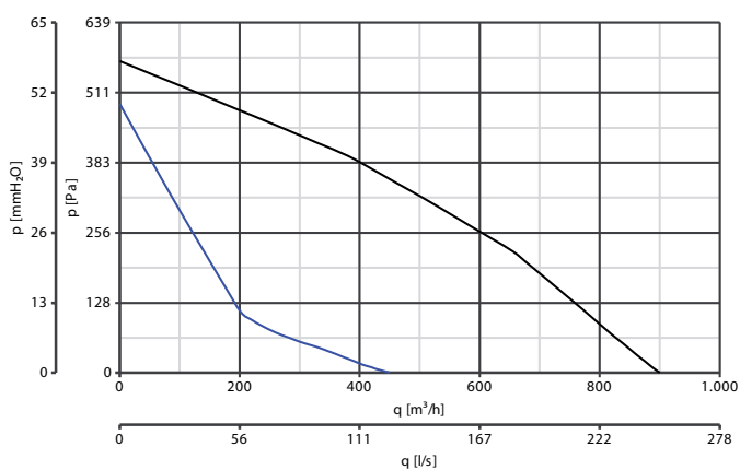
CA 315 MD E RF CODE 16187
