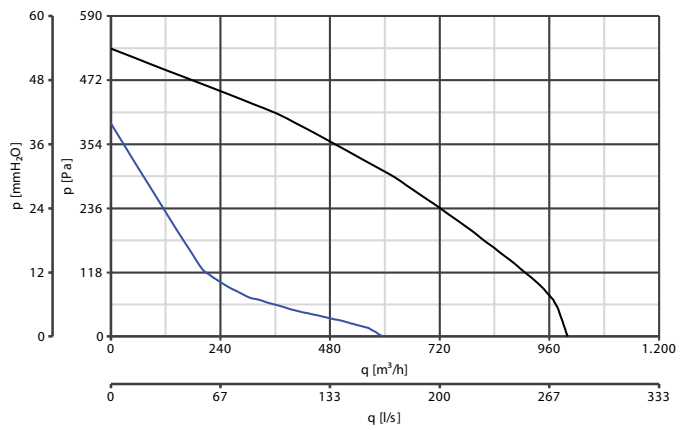
CA 250 MD E W CODE 16136
