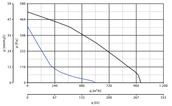
CA 250 MD E CODE 16166
