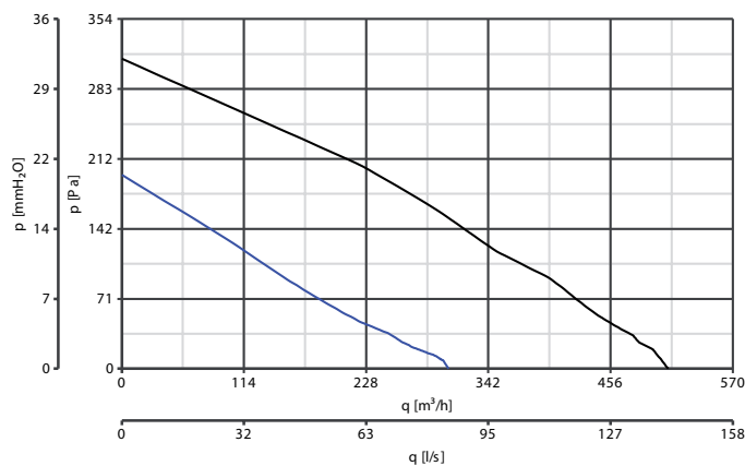
CA 160 MD E W CODE 16134
