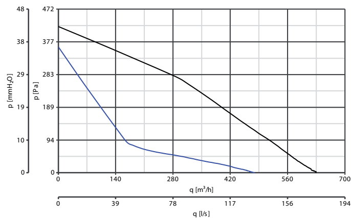
CA 200 MD E W CODE 16135
