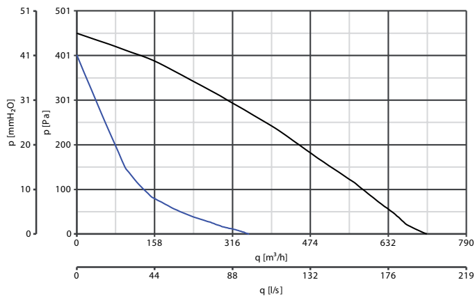
CA 200 MD E RF CODE 16185
