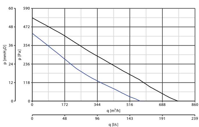
CA 200 MD CODE 16155
