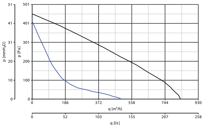
CA 315 MD E CODE 16167
