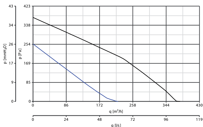
CA 150 MD E RF CODE 16183
