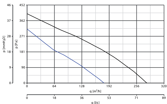
CA 150 Q MD E RF CODE 16142
